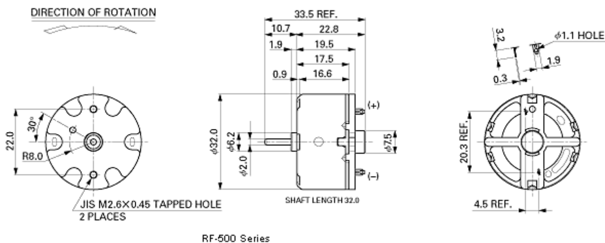
RF-500 Mechanical drawing
