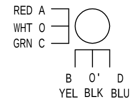
Wiring Diagram
